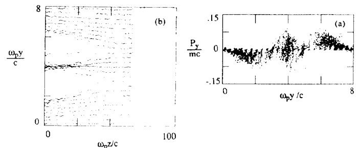
Fig. 6. Phase space and real space trajectories in the double plasma wave wigglers.
