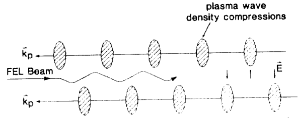
Fig. 2. Geometry of plasma wiggler FEL scheme 2 ( \vec{v}_b \parallel \vec{k}_p ).
