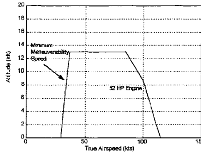
Figure 3: Flight Envelope
